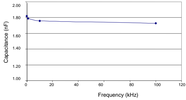
Figure 4. BTO/Epoxy nanocomposite dielectric capacitance (nF) as a function of frequency (KHz) (5 μm nanocomposite thickness).
