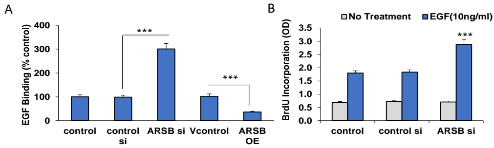
Figure 5. Increased BrdU incorporation in prostate stem cells in response to exogenous EGF following ARSB.
