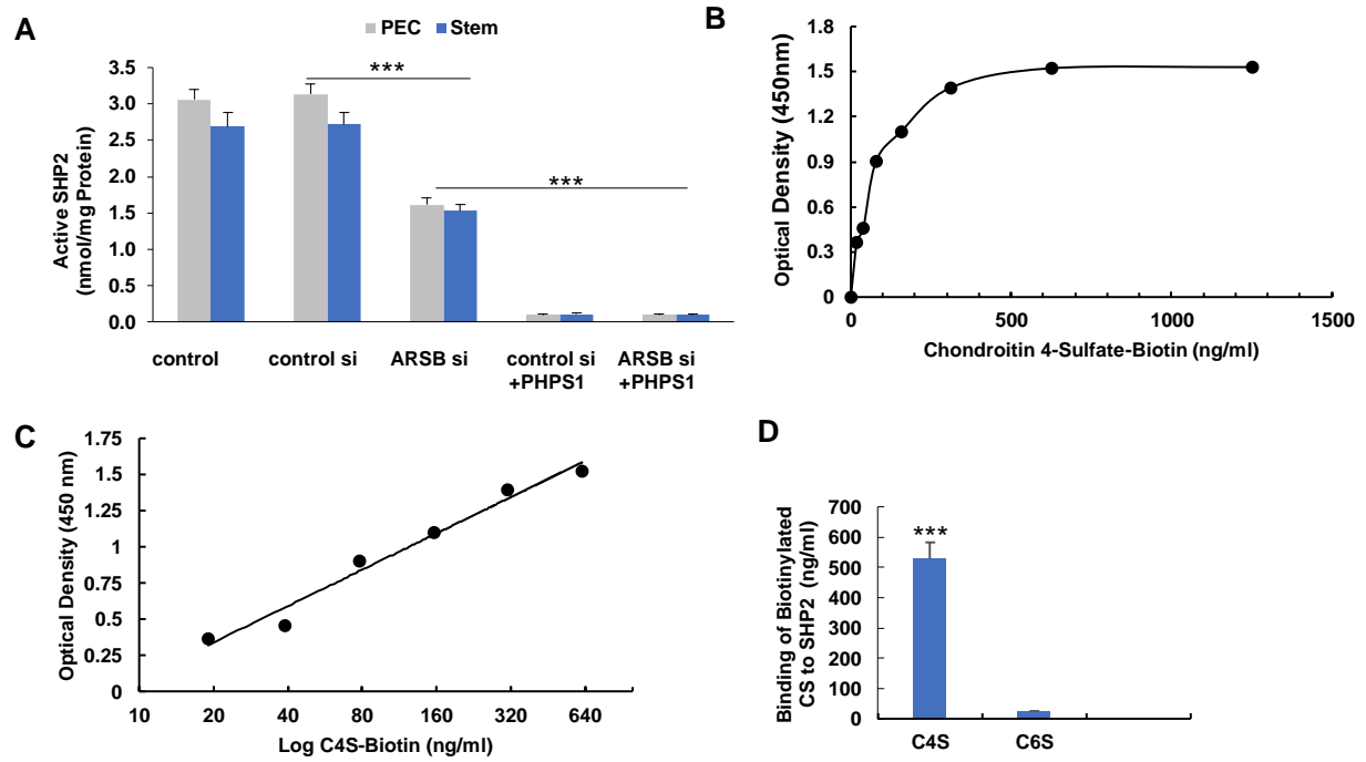
Figure 2. SHP2 Activity is reduced following ARSB silencing; attributable to increased binding with C4S.
