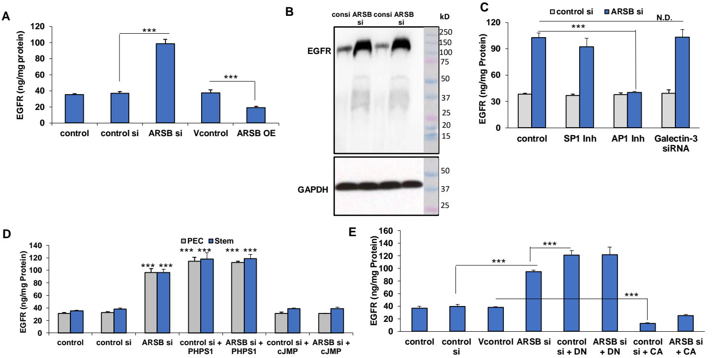
Figure 1. EGFR is increased following decline in ARSB or in SHP2 and is reduced by AP1 inhibition, but unaffected by galectin-3 silencing.
