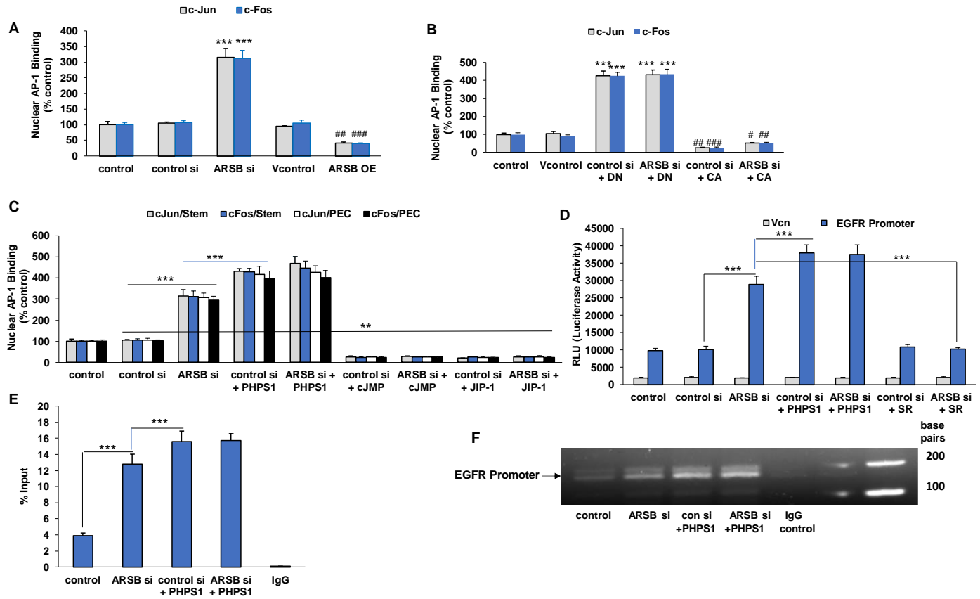
Figure 4. Increased nuclear AP-1 binding and EGFR promoter activation following ARSB silencing or SHP2 inhibition.
