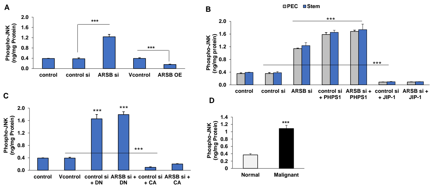
Figure 3. Phospho-JNK is increased in prostate stem cells and prostate tissue following ARSB silencing or SHP2 inhibition.
