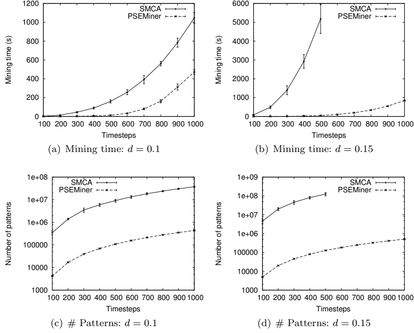
Fig. 12. The performance of SMCA compared to our algorithm.
