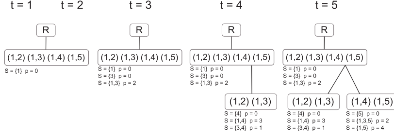
Fig. 6. The pattern tree at each timestep for the dynamic network shown in Figure 3, considering only edges for brevity.
