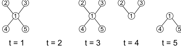
Fig. 3. An example of a dynamic network with 2 PSEs at \sigma = 3 .
