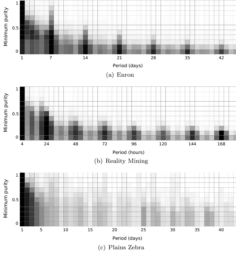
Fig. 10. Pattern density at each minimum purity threshold. Each row shows the distribution of pattern periods for patterns with purity at or greater than the y-axis value. Darker cells indicate more patterns.
