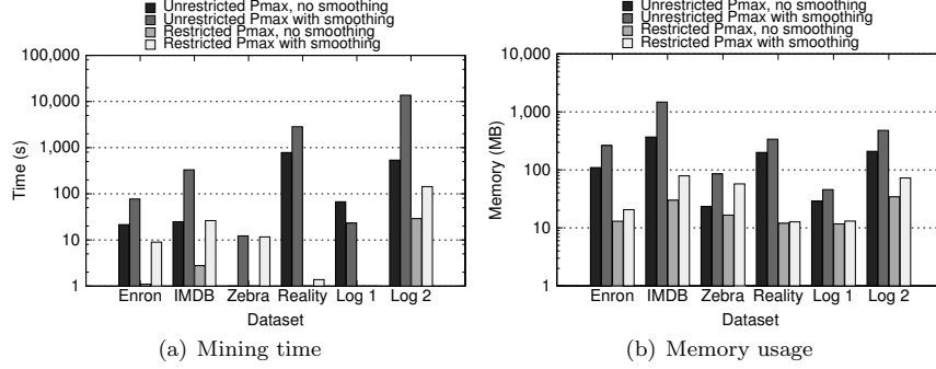
Fig. 7. Performance of the periodic subgraph mining algorithm at \sigma = 3 , shown with an exponential y-axis.
