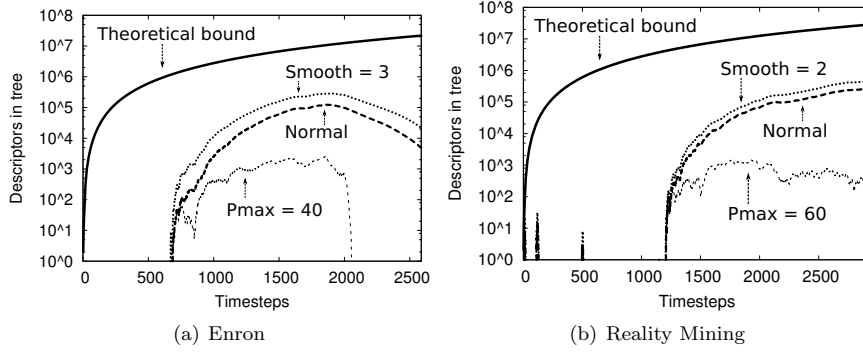
Fig. 8. Number of pattern tree descriptors with no smoothing or restrictions on period ('normal'), and for various smoothing and P_{\max} values, compared to the theoretical bound.
