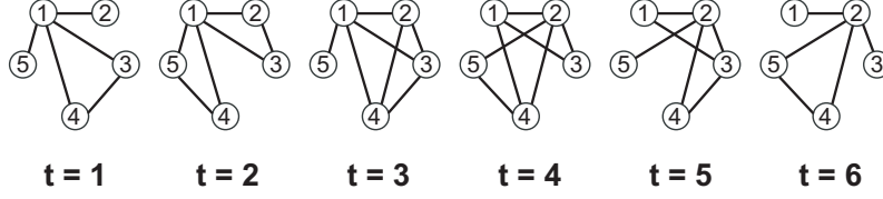
Fig. 5. An example of a worst case dynamic network for mining PSEs at \sigma = 3 .
