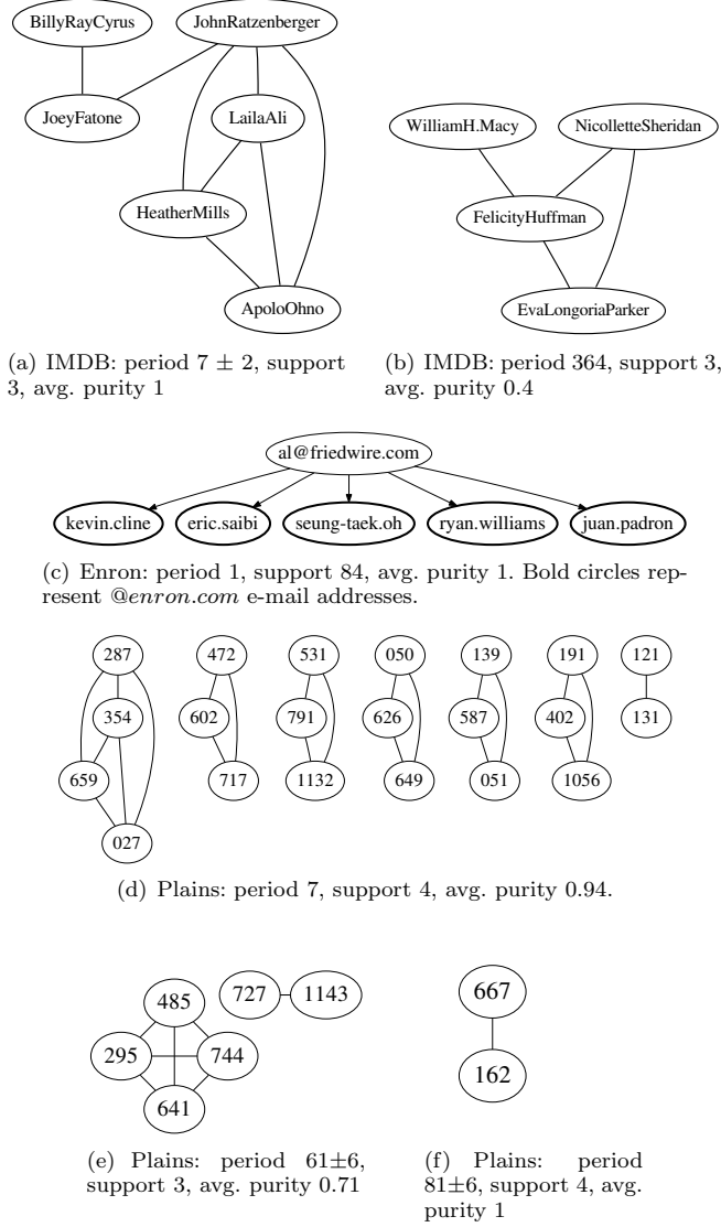
Fig. 11. Examples of some interesting periodic subgraphs.
