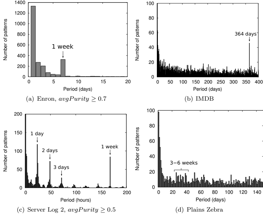
Fig. 9. Number of patterns at each period.
