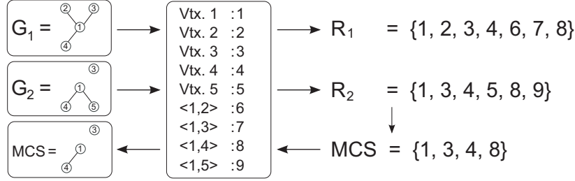
Fig. 2. The correspondence between graph and set representations for graphs with unique vertex labels. The example demonstrates the computation of the maximal common subgraph of two graphs using set representation.
