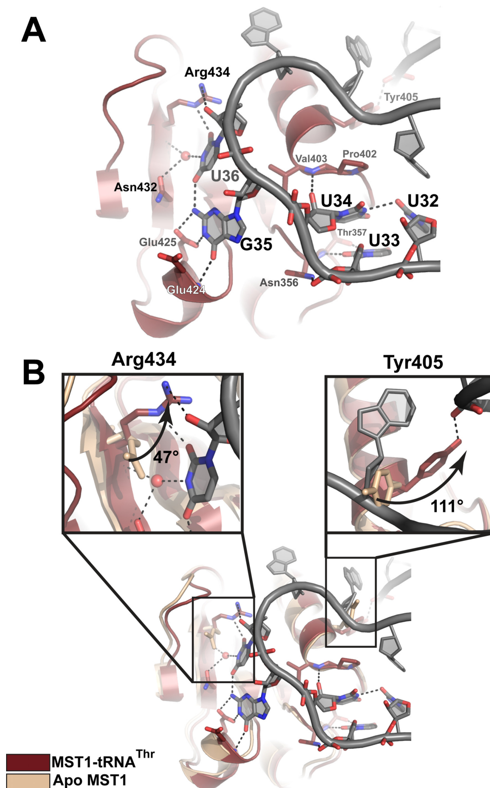
Figure 4. Recognition of the anticodon sequence and structural rearrangements in the anticodon-binding domain of MST1 upon complex formation. (A) The first position in the anticodon sequence, U34, is not specifically recognized by MST1. Instead, Thr357 recognizes U33, the base upstream of the anticodon. The second base, G35, is recognized by the backbone amide of Glu424 and Glu425, whereas the third position, U36, is recognized by Asn435, the backbone atoms of Arg434, and a water molecule. The backbone atoms of MST1 and tRNA are red and grey, respectively. (B) Superimposition of apo MST1 (PDB ID 3UGQ; beige) onto the MST1-tRNA complex (red and grey) reveals structural rearrangements in the anticodon-binding domain upon tRNA binding. The first inset highlights the movement of Arg434 that is important for recognition of U36. The side chain of Arg434 rotates \sim 47^\circ and translates \sim 1.4 Å toward the tRNA. The second inset shows rotation ( \sim 111^\circ ) of Tyr405. This movement positions the side-chain hydroxyl within the H-bonding distance from the sugar-phosphate backbone of A26 in the anticodon stem.
