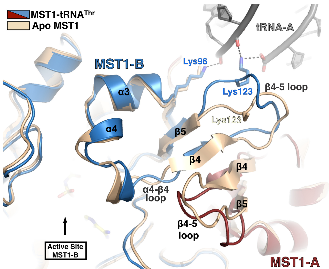
Figure 3. Cross-subunit interactions with the acceptor stem induce a conformational rearrangement in the active-site lid. Superimpositioning of the apo-MST1 structure (PDB ID: 3UGQ; beige) onto the MST1-tRNA complex (red, blue and grey) reveals structural rearrangements in the catalytic domain upon tRNA binding. Residues Lys96 and Lys123 from the MST1-B monomer (blue) interact with the sugar-phosphate backbone of the acceptor stem of the tRNA primarily bound to the MST1-A monomer (red). These interactions presumably induce to a conformational change in flexible loops \beta 4 - \beta 5 and \alpha 4 - \beta 4 that result in movement of the helix \alpha 4 and thus widening of the active-site lid to accommodate the 3' end of tRNA. This is a possible mechanism of allosteric regulation that allows the active site of one monomer to 'sense' when tRNA is bound to the other monomer.
