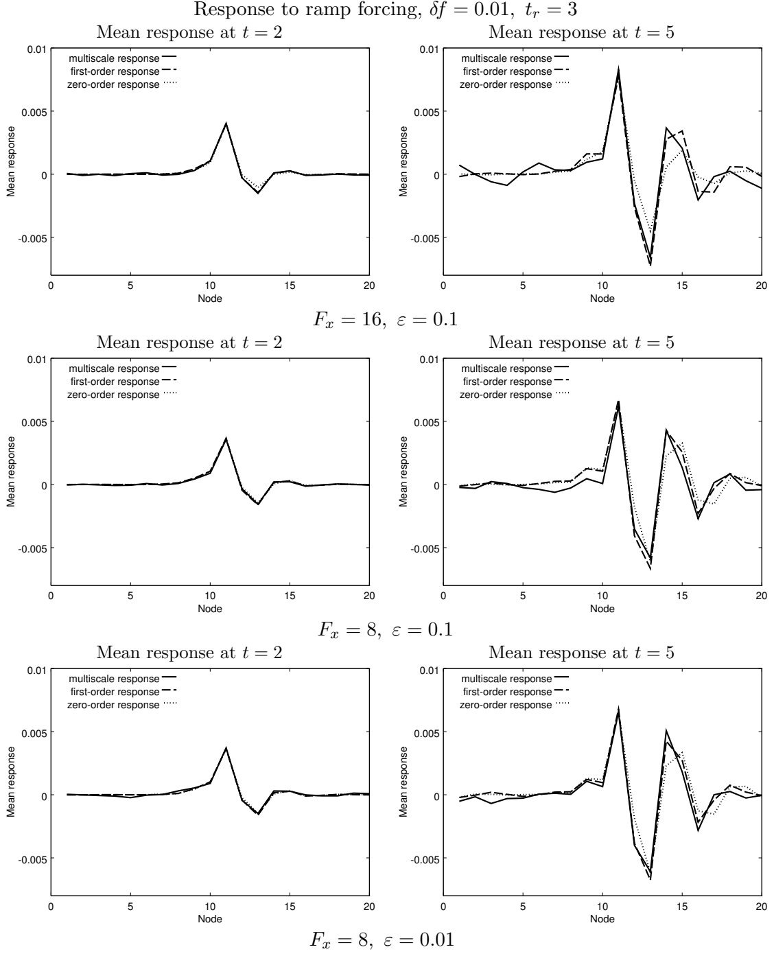
Figure 10. Snapshots of the mean response \delta \bar{\mathbf{x}}(t) to small ramp forcing
