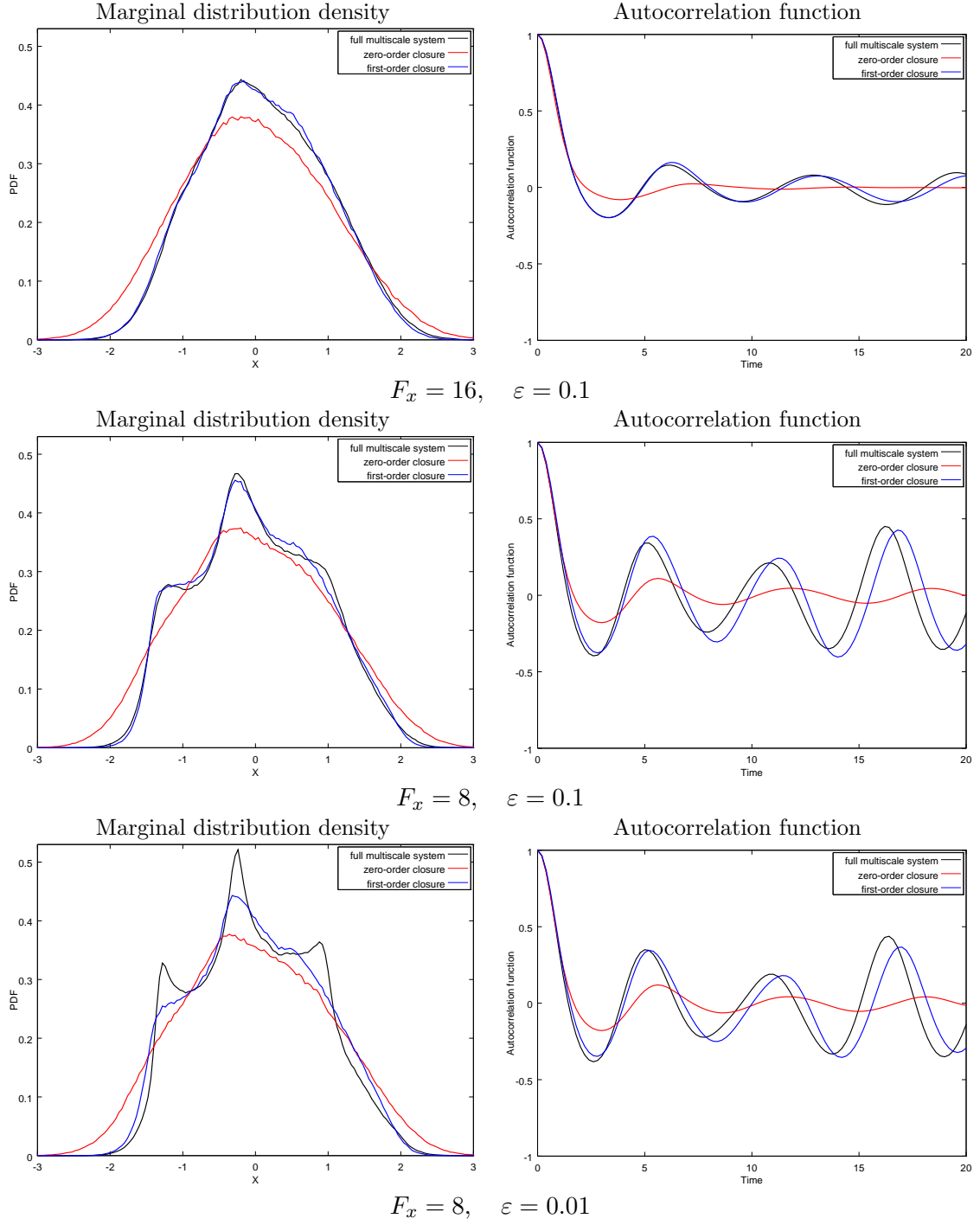
Figure 1. Marginal distribution densities and autocorrelation functions of slow variables.
