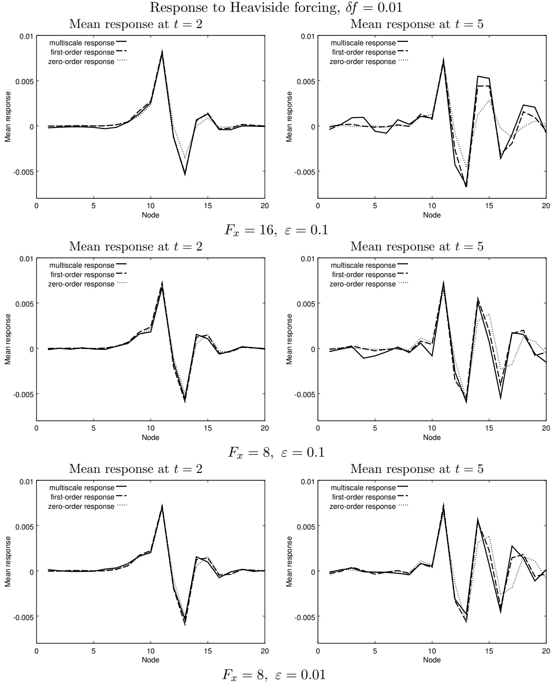
Figure 8. Snapshots of the mean response \delta \bar{\mathbf{x}}(t) to small Heaviside forcing
