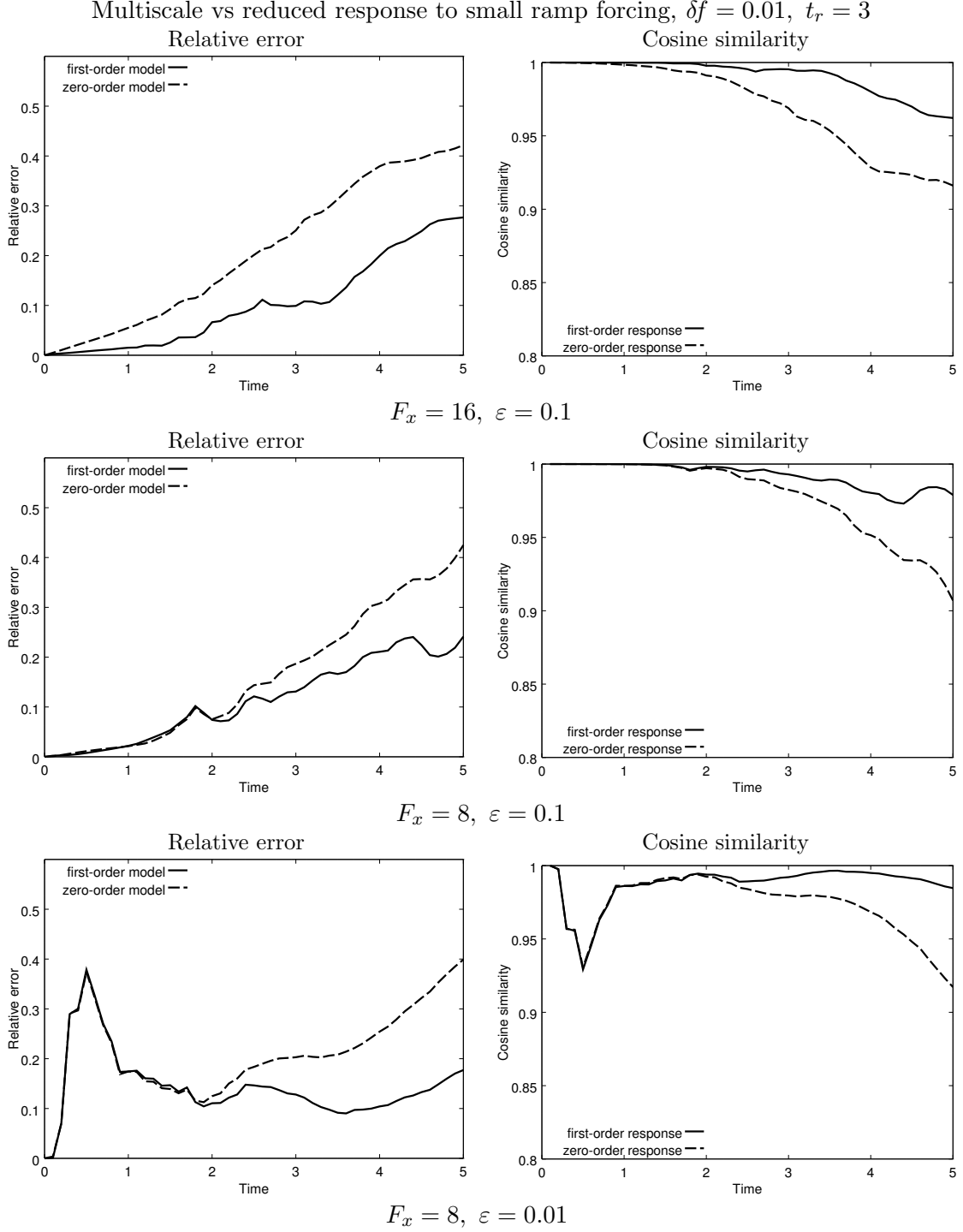
Figure 14. Comparison of multiscale and reduced system mean responses \delta \bar{\mathbf{x}}(t) to small ramp forcing with t_r = 3 using relative distance (8.3) and cosine similarity (8.4).
