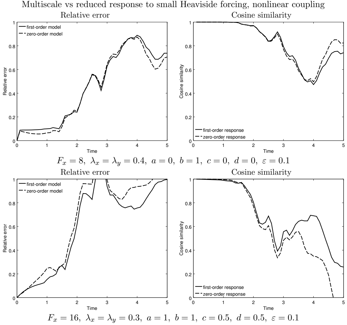
Figure 16. Comparison of multiscale and reduced system mean responses \delta\bar{\mathbf{x}}(t) to small Heaviside forcing for Lorenz 96 system with nonlinear coupling.
