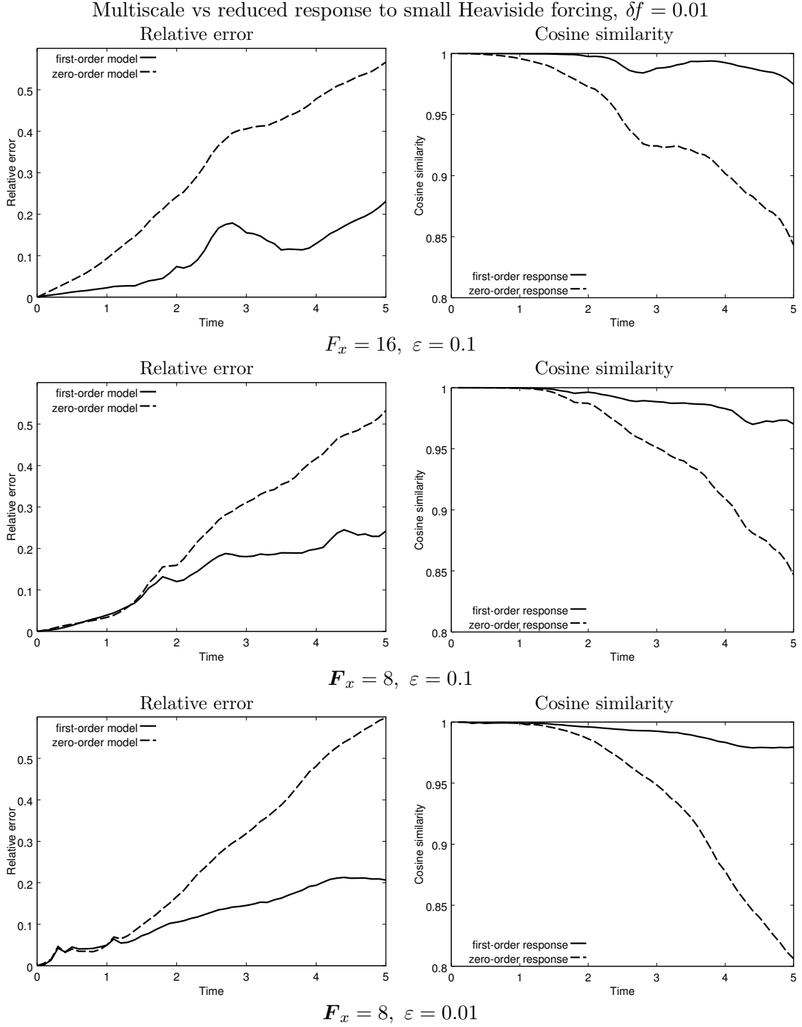
Figure 12. Comparison of multiscale and reduced system mean responses \delta \bar{x}(t) to small Heaviside forcing using relative distance (8.3) and cosine similarity (8.4).
