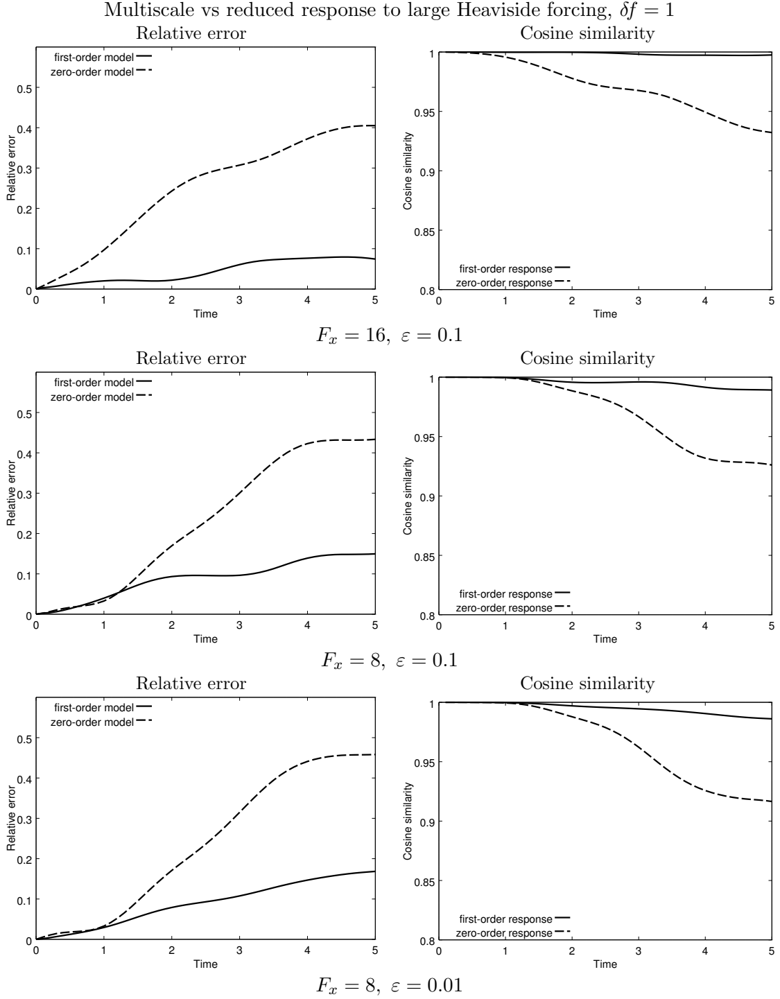
Figure 13. Comparison of multiscale and reduced system mean responses \delta \bar{\mathbf{x}}(t) to large Heaviside forcing using relative distance (8.3) and cosine similarity (8.4).
