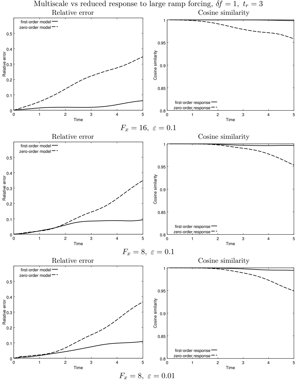
Figure 15. Comparison of multiscale and reduced system mean responses \delta \bar{\mathbf{x}}(t) to large ramp forcing with t_r = 3 using relative distance (8.3) and cosine similarity (8.4).
