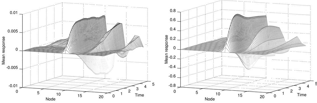
Figure 7. Response of \langle \mathbf{x} \rangle ( b(\mathbf{x}) = \mathbf{x} in (5.5)) to Heaviside step forcing \delta f = 0.01 (left) and \delta f = 1 (right) at node x_{11} in a chaotic regime of the two-time rescaled Lorenz 96 system.
