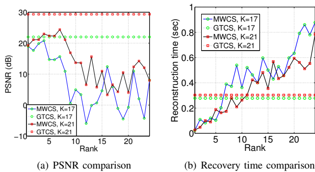
Fig. 12. PSNR comparison of GTCS-P with MWCS on compressible video when m = 17 , using 0.36 normalized number of samples and m = 21 , using 0.67 normalized number of samples. The highest PSNR of MWCS with estimated tensor rank varying from 1 to 24 appears when Rank = 4 and Rank = 7 respectively.
