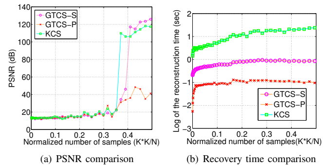
Fig. 1. PSNR and reconstruction time comparison on sparse image.
