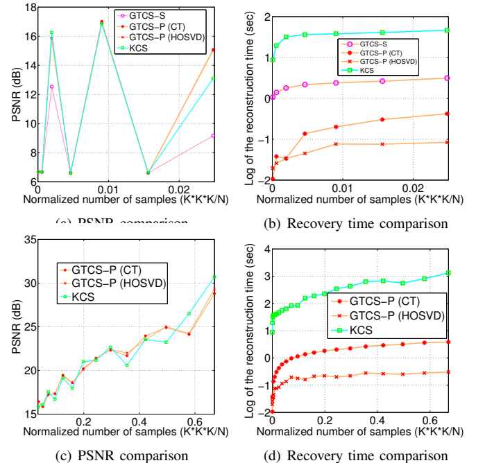
Fig. 9. PSNR and reconstruction time comparison on susie video.
