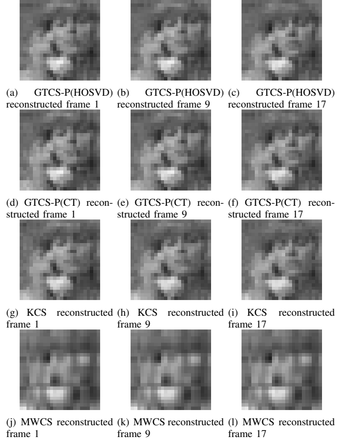
Fig. 11. Reconstructed video frames when m = 21 using 0.67 normalized number of samples by GTCS-P (HOSVD, PSNR = 29.33 dB), GTCS-P (CT, PSNR = 28.79 dB), KCS (PSNR = 30.70 dB) and MWCS (Rank = 4, PSNR = 22.98 dB).
