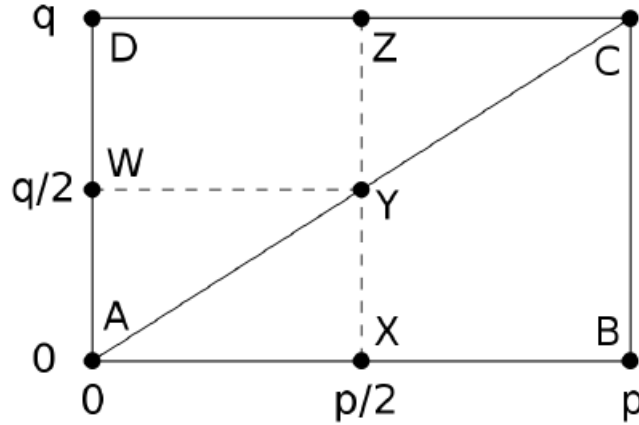
Figure 2: The triangle ABC .
