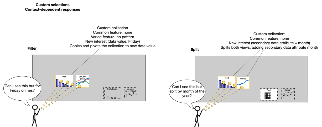
Figure 30: Context dependent responses to the same referential request. Two different cases, with two different responses, that depend on the targeted views, and an assessment of their common and varied features. In these cases, the user indicated views that did not have clear conserved features, but Ditto can respond with filter and split actions in some cases.
