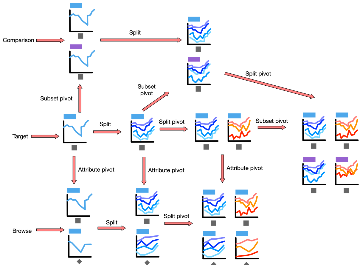
Figure 18: This is a second example of a set of referential pivot paths. We show alternate routes to different collections of views. The types on the side and top, are direct question types, and the transitions are different types of referential actions.
