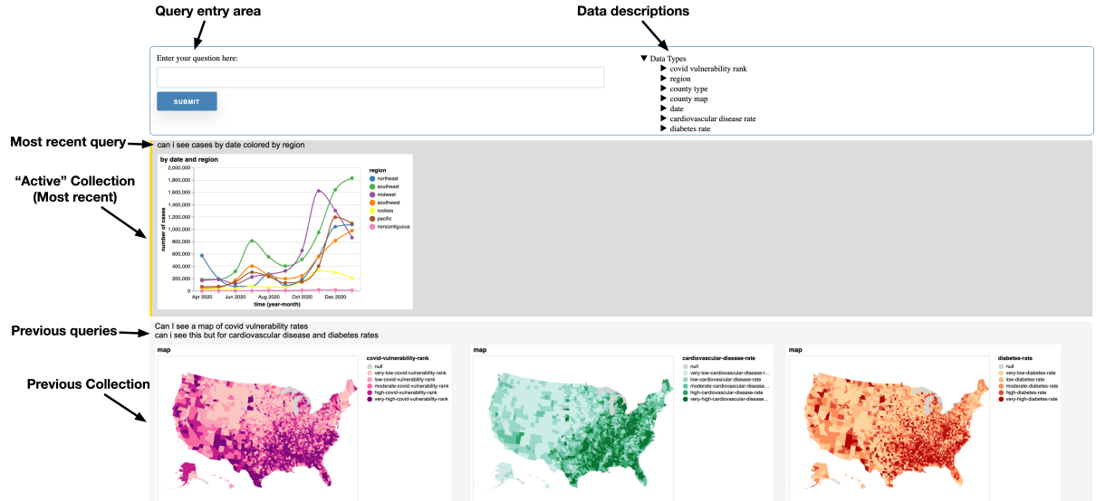
Figure 20: The traverse user interface consists in a query entry area, an interactive data description area, a query and view collection response area, with previous collections shown in a scrolling history. The examples shown above are from the COVID19 data and problem description which is described in detail in Appendix A.
