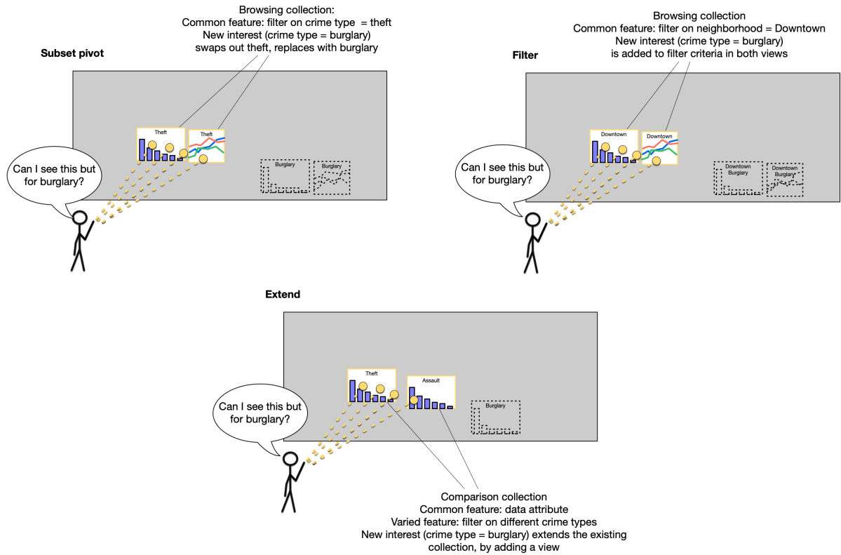
Figure 28: Context dependent responses to the same referential request, involving new data values of interest. Three different cases, with three different responses, that depend on the targeted views, and an assessment of their common and varied features
